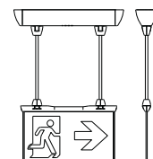
Rod Suspension 48cm (ISO30061) (O-ESA-PS30)
